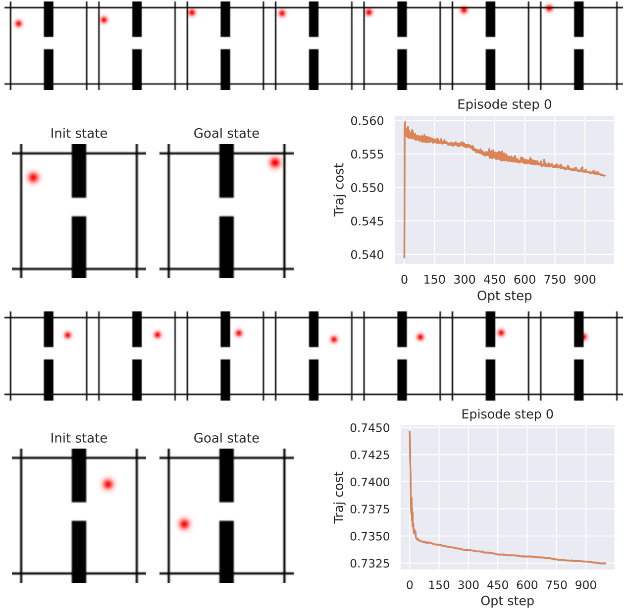
Figure 10: Two typical failure cases with the Gradient-Descent (GD) planner on the Wall task. For each failure case, we show: (top) the planned trajectory visualization, (bottom left) initial and goal states, (bottom right) planning cost evolution throughout gradient descent iterations. First failure case (top 3 subfigures): the agent finds a local planning cost minimum by going to the borders of the image when starting close to them. Second failure case (bottom 3 subfigures): the agent goes into the wall without being able to pass the door.
