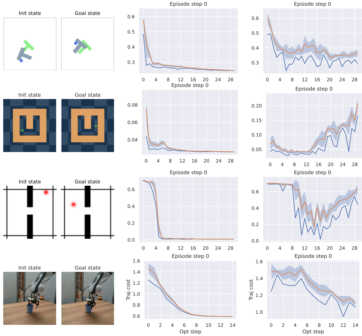
Figure 17: Convergence of planning optimization for all 2D environments and DROID. The model evaluated is the base WM model, at the end of training. Left: episode initial and goal state. Center: CEM planner. Right: NG planner. We display the planning cost of the best trajectory throughout the optimization steps.
